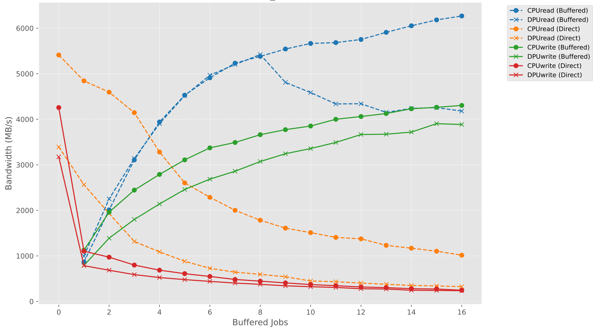
Bandwidth vs Buffered Jobs (direct1_bufferedN) - SEQ (CPU vs DPU)
